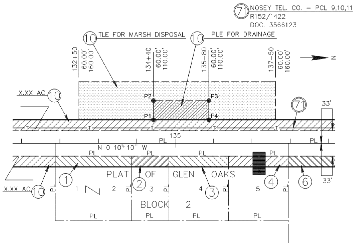
Figure 1.6 Subdivision & Utility Interest Example
